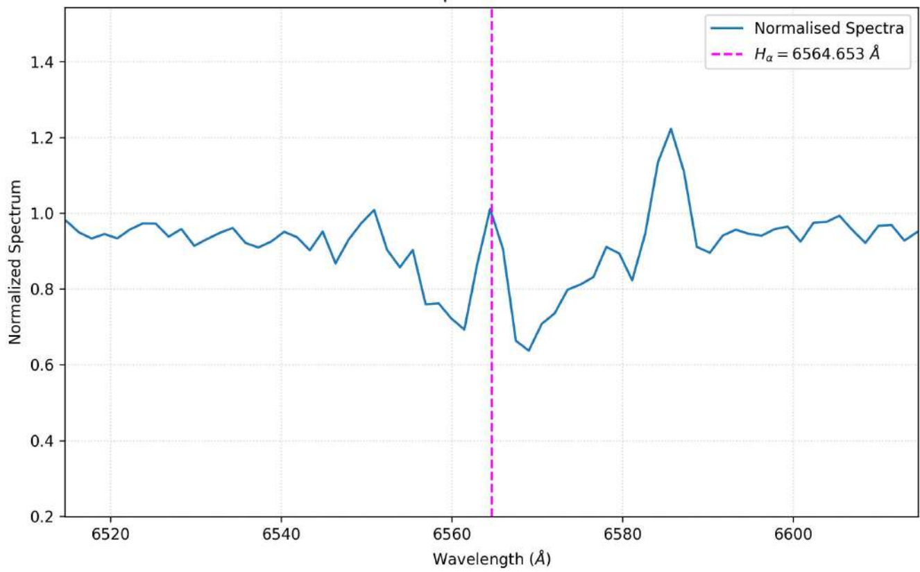
Normalised Spectrum for 892915182
