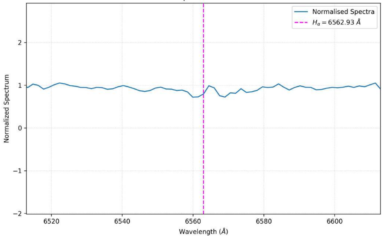
Normalised Spectrum for 966211211
