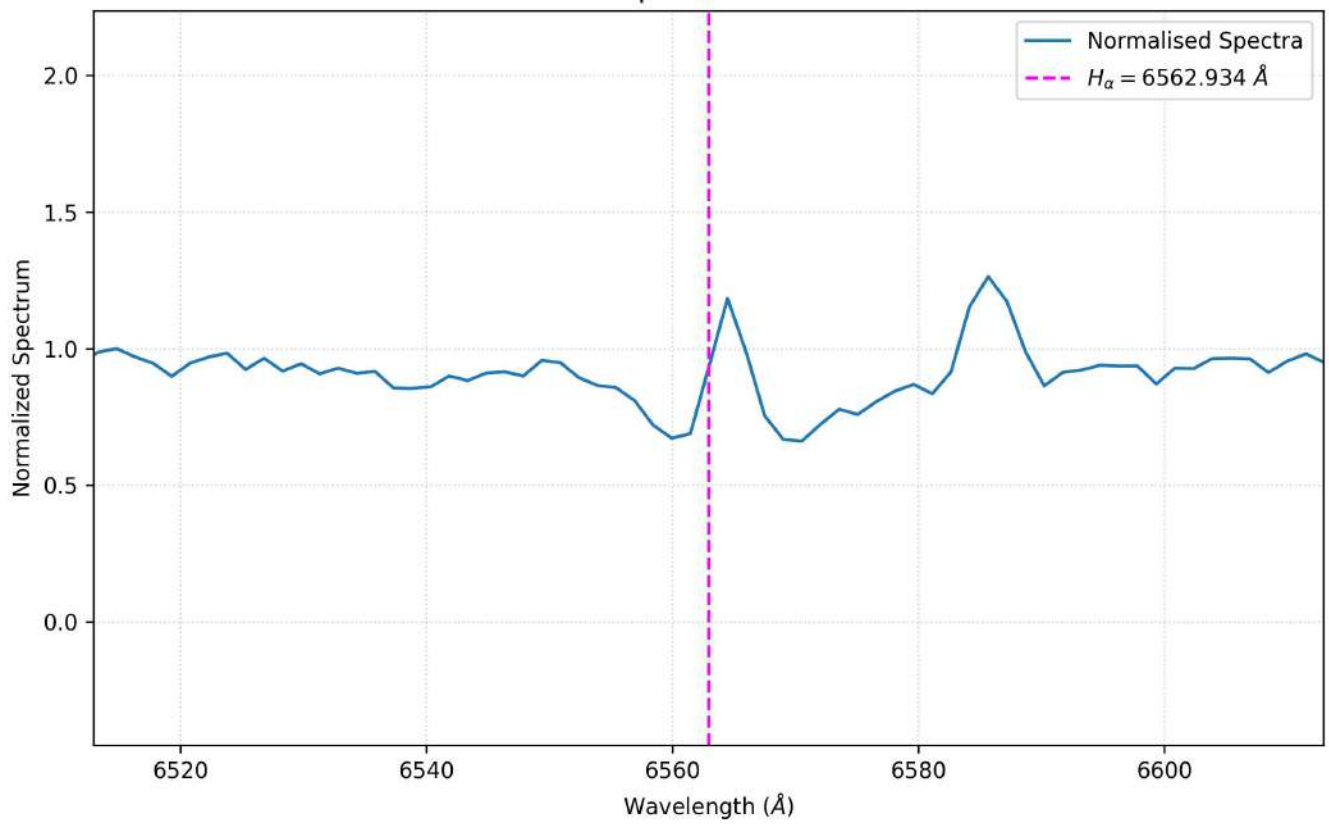
Normalised Spectrum for 892904135
