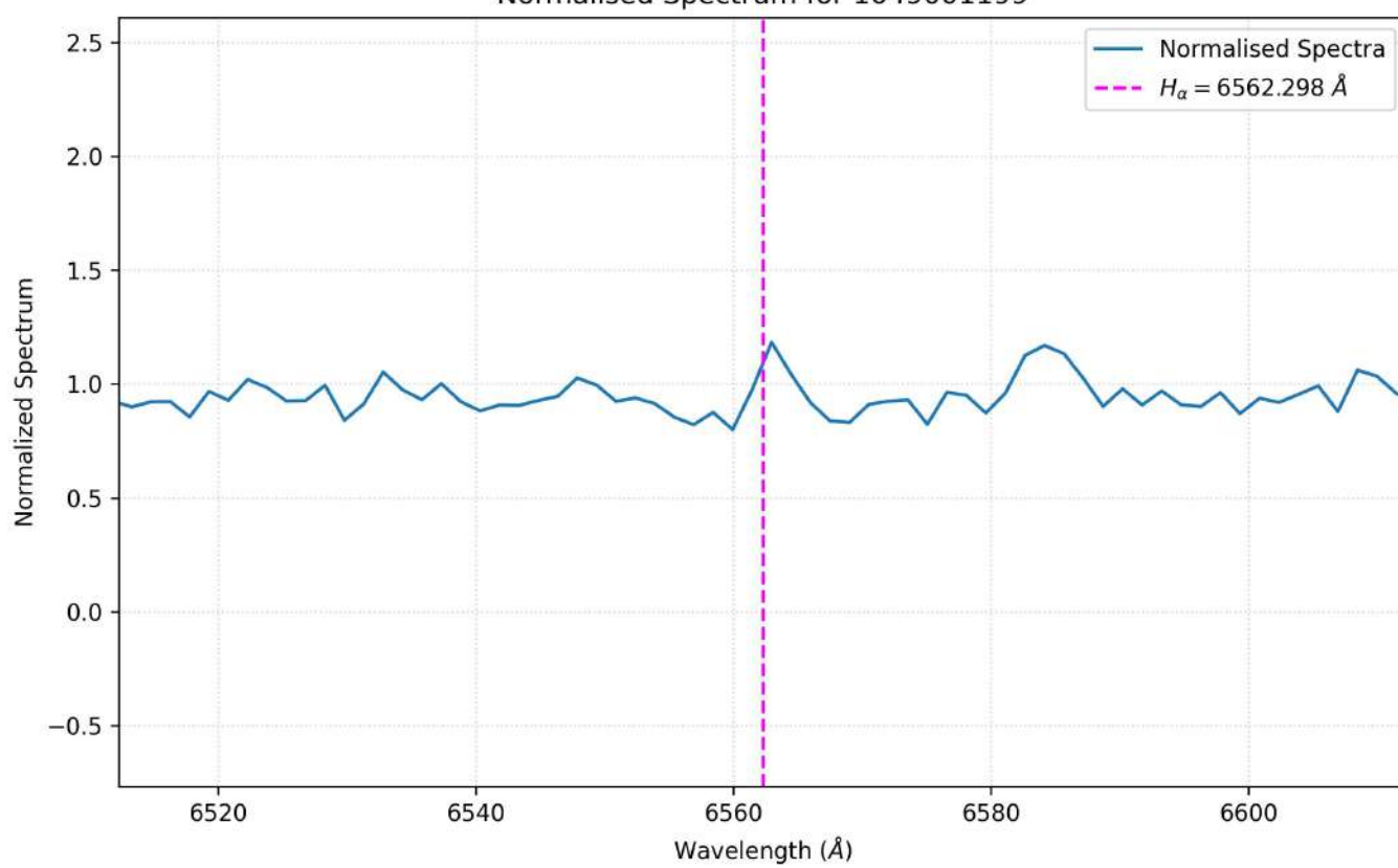
Normalised Spectrum for 1049001199
